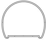
Excell Round Top Sleeve HEIGHT: 2 1/16" WIDTH: 2 7/16" ALLOY: 6063-T5
