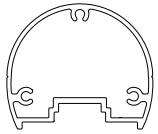
Excell Round Top Rail (Welded Picket) HEIGHT: 2 1/16" WIDTH: 2 7/16" ALLOY: 6063-T5
