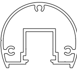
Excell Round Top Rail (Component Glass) HEIGHT: 2 1/16" WIDTH: 2 7/16" ALLOY: 6063-T5
