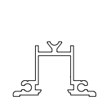
Receiver Channel (Component Glass) HEIGHT: 1 5/16" WIDTH: 2" ALLOY: 6063-T5
