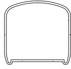
Excell Square Top Sleeve HEIGHT: 2 1/16" WIDTH: 2 3/16" ALLOY: 6063-T5
