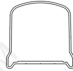
Standard Square Top Sleeve HEIGHT: 2 3/8" WIDTH: 2 3/8" ALLOY: 6063-T5
