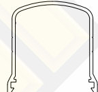
Standard Square Top Rail HEIGHT: 2 1/4" WIDTH: 2 3/16" ALLOY: 6063-T5
