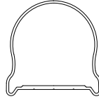
Standard Round Top Sleeve HEIGHT: 2 3/8" WIDTH: 2 3/8" ALLOY: 6063-T5
