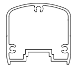
Excell Square Top Rail (Welded Picket) HEIGHT: 2 1/16" WIDTH: 2 3/16" ALLOY: 6063-T5
