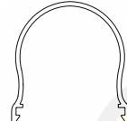
Standard Round Top Rail HEIGHT: 2 1/4" WIDTH: 2 3/16" ALLOY: 6063-T5
