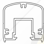
Excell Square Top Rail (Component Glass) HEIGHT: 2 1/16" WIDTH: 2 3/16" ALLOY: 6063-T5
