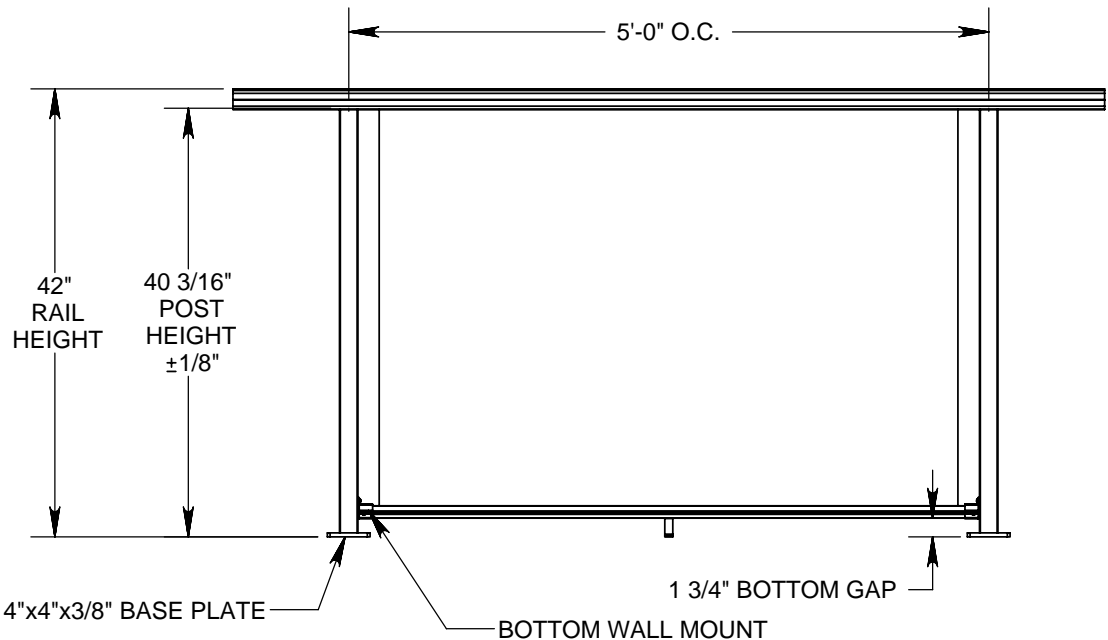
COMPONENT GLASS BOTTOM RAIL
