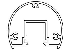
EXCELL ROUND COMPONENT GLASS TOP RAIL
